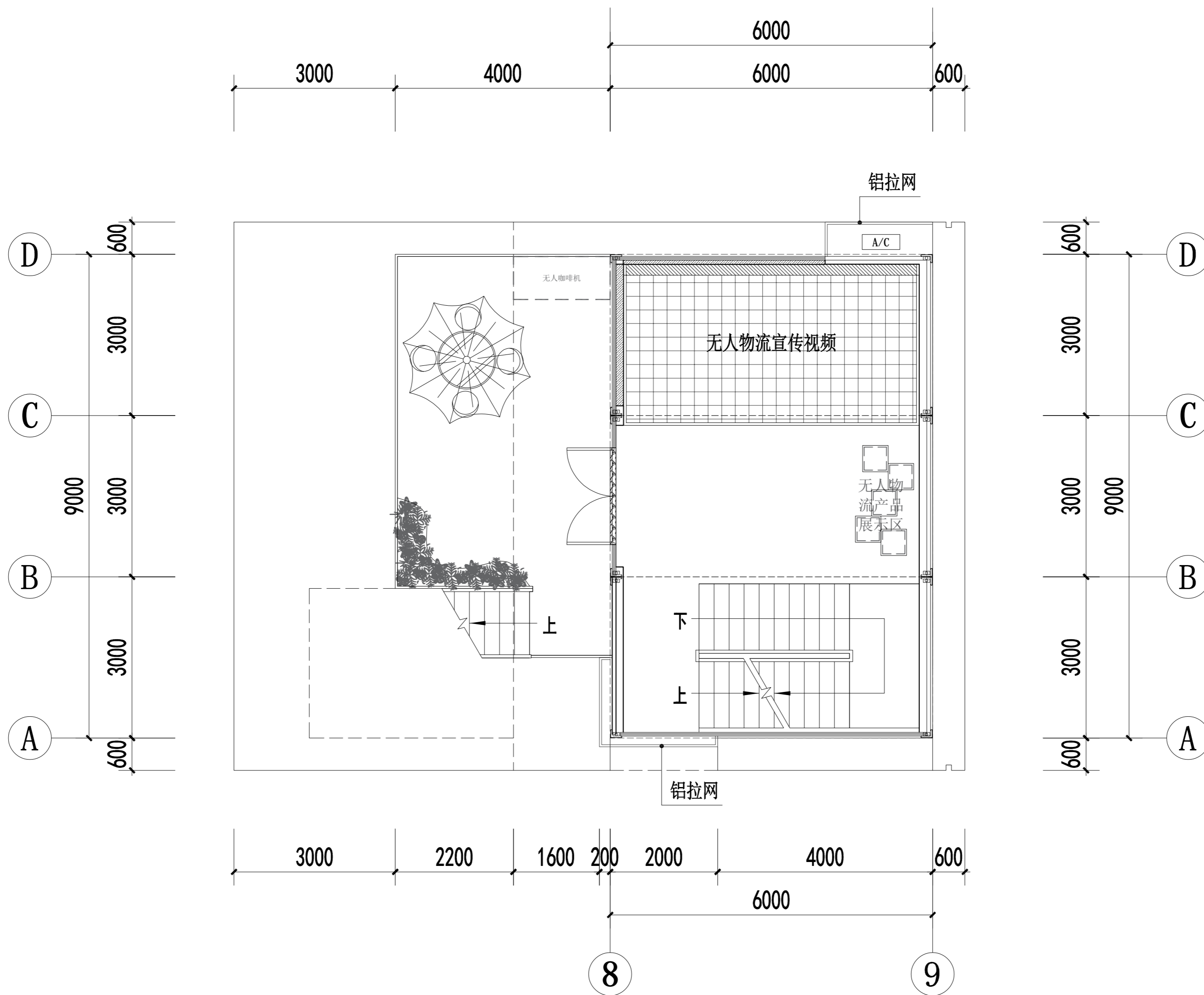
C栋二层平面图 (54m 2 )
